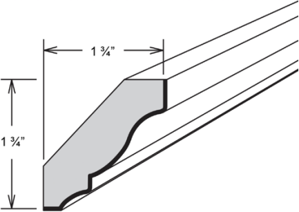
Crown ■CM8
