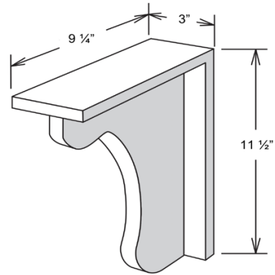
Curved Corbel
