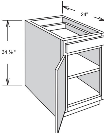
1 Door 1 Drawer
