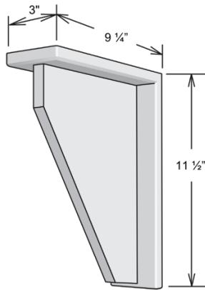
Angled Corbel
