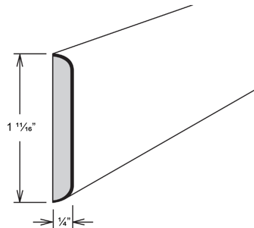
Wide Batten
