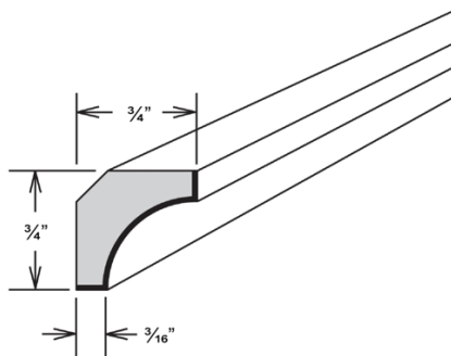
Inside Corner
