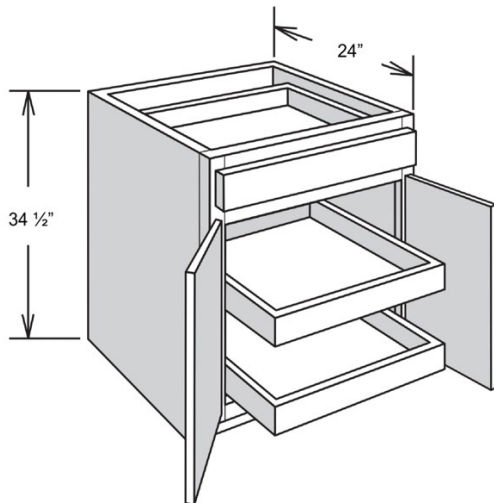
2 Sliding Shelves
